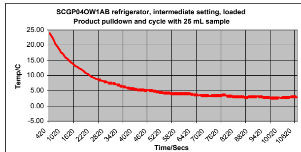
Typical performance characteristic with load
