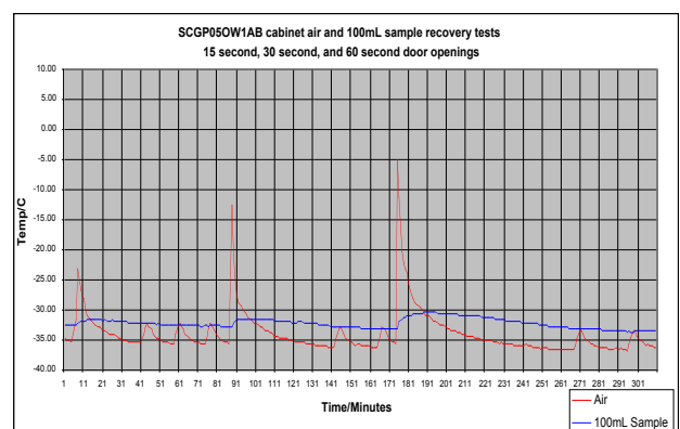
Typical performance, door opening recovery
