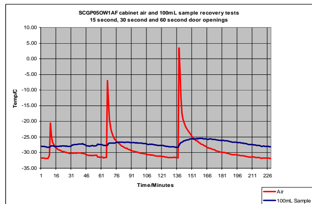
Typical performance, door opening recovery
