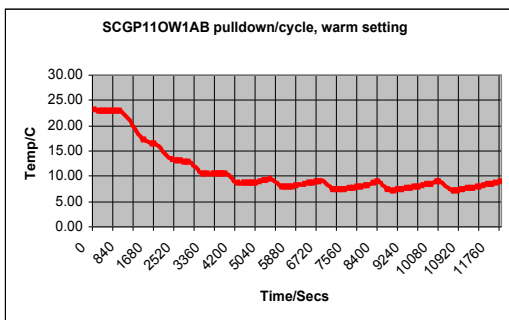
Typical performance characteristic, unloaded
