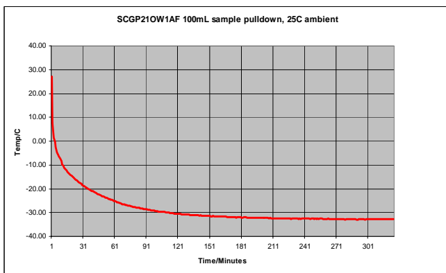
Typical performance product pull-down
