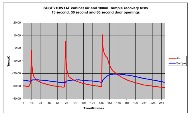
Typical performance, door opening recovery
