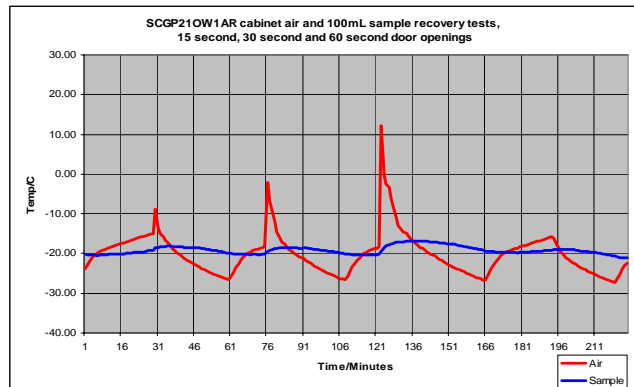
Typical performance, door opening recovery
