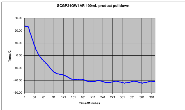
Typical performance ambient pull-down
