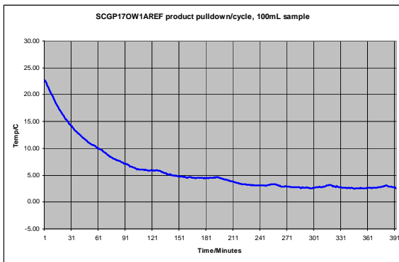
Typical performance ambient pull-down
